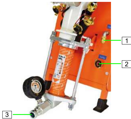
Abb. 20: Anschlüsse
